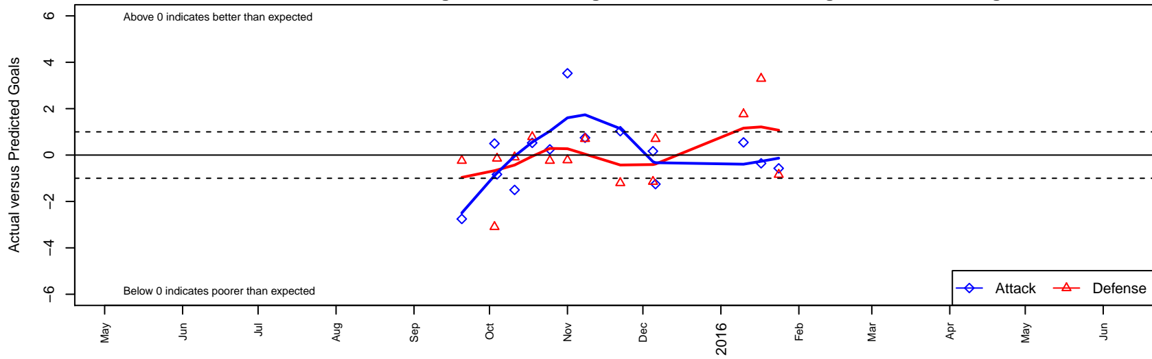
Norpoint AC Milan B98 Dots are actual minus expected GF (blue circles) and GA (red triangles). Blue line is smoothed change in attack strength. Red is smoothed change in defense strength.
